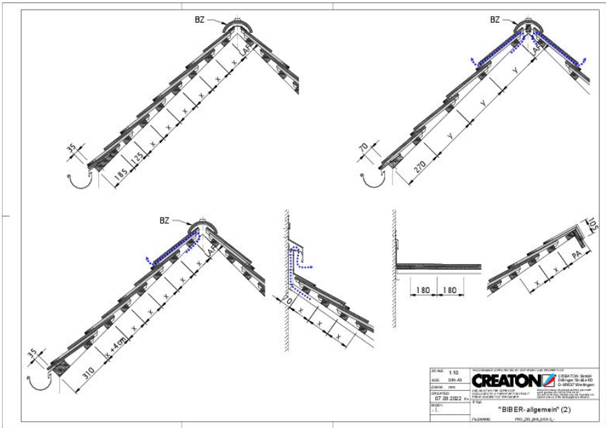
Drawing KLASIK general view GES-2
