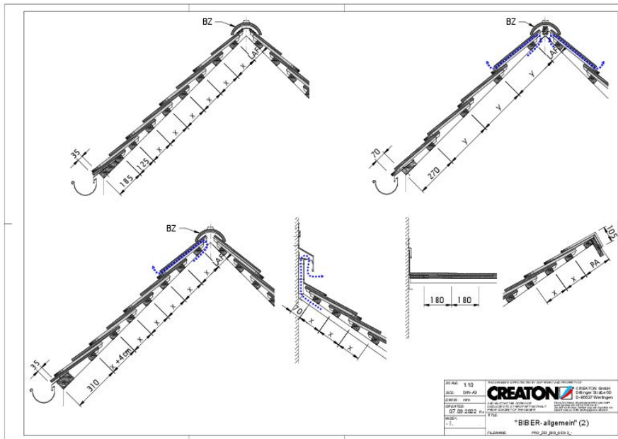
Drawing KLASSEK general view GES-2
